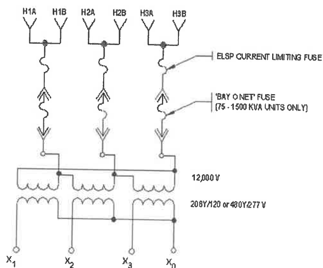
Figure 2 Internal Schematic
